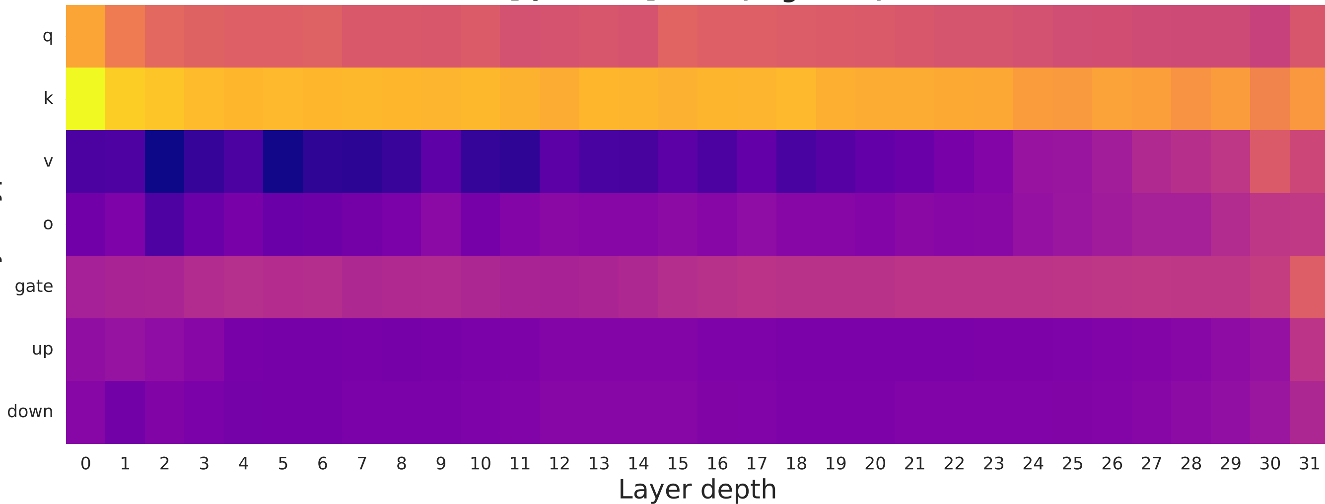
[QTIP-4bit] MSE (Log scale)
